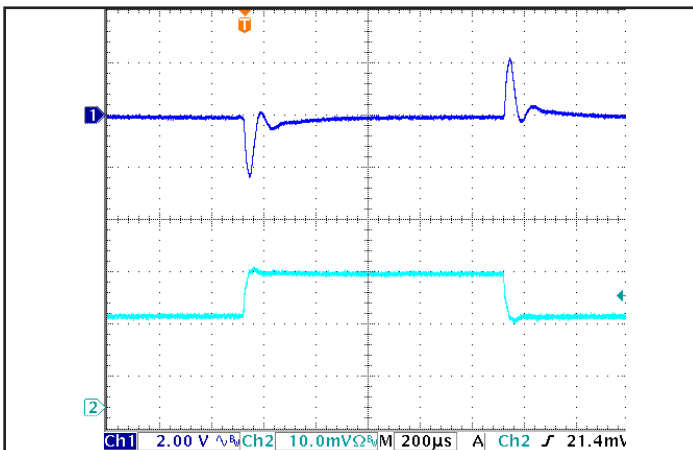
Figure 5: Output voltage response to step-change in load current (66% -100% -66% of I_{out(max)} ; dI/dt = 0.2 \text{ A}/\mu\text{s} ). Load cap: 1 \mu\text{F} ceramic capacitor. Ch 1: V_{out} (2 V/div), Ch 2: I_{out} (2 A/div).
