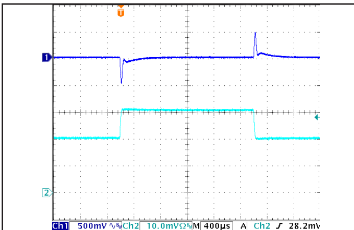
Figure 5: Output voltage response to step-change in load current (66% -100% -66% of I out (max); dI/dt = 0.2 A/us). Load cap: 15 μF tantalum and 1 μF ceramic capacitors. Ch 1: V out (500 mV/div), Ch 2: I out (5 A/div).
