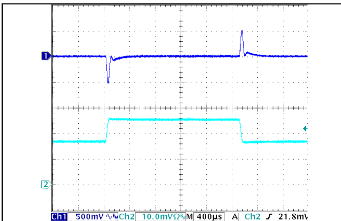
Figure 5: Output voltage response to step-change in load current (66% -100% -66% of I out (max); dI/dt = 0.2 A/µs). Load cap: 15 µF tantalum and 1 µF ceramic capacitors. Ch 1: V out (500 mV/div), Ch 2: I out (5 A/div).
