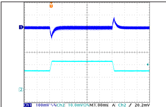
Figure 5: Output voltage response to step-change in load current (66% -100% -66% of I out(max) ; dI/dt = 0.2 A/μs). Load cap: 15 μF tantalum and 1 μF ceramic capacitors. Ch 1: V out (100 mV/div), Ch 2: I out (20 A/div).
