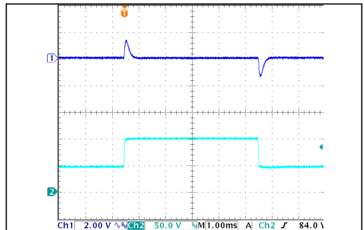
Figure 6: Output voltage response to step-change in input voltage (nominal to maximum, 250 V/ms). Load cap: 1 \mu\text{F} ceramic capacitor. Ch 1: V_{out} , Ch 2: V_{in} .
